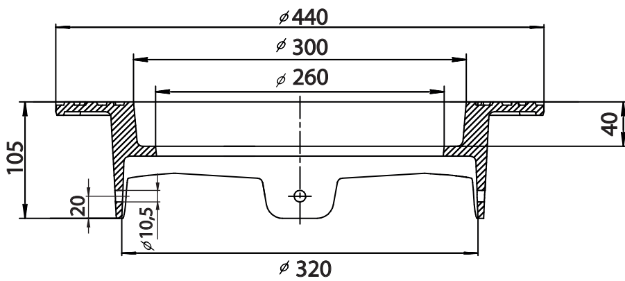
Frame art. 315 Fnl D400
